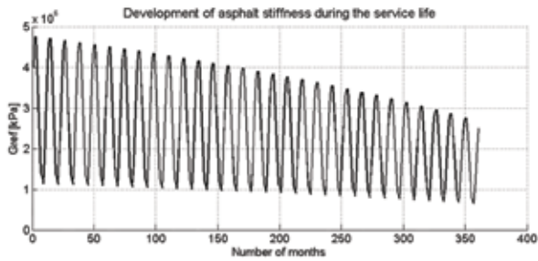
Figure 5a: Decrease of temperature-dependent asphalt stiffness (shear modulus G) during runway 14/32 service life
