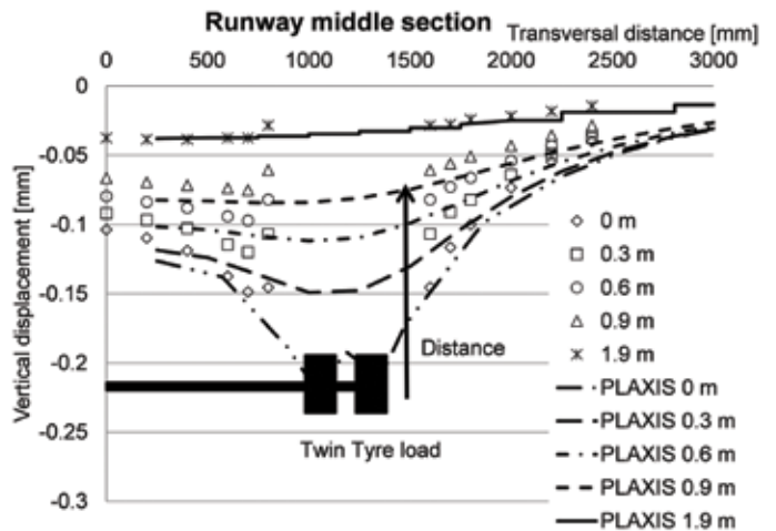
Figure 7: Measured (dots) and back-calculated (lines) deflection bowl induced by a track load (twin tyre). The test was carried out on runway 16/34 of Zürich international airport
