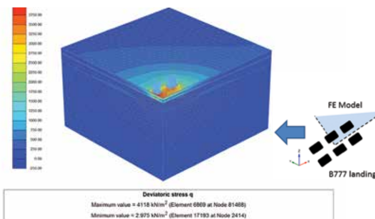
Figure 4a: Symmetrical 3D finite element model of 1/4 of the pavement and load (B777-300ER landing gear). The plot shows the calculated deviatoric stresses q
