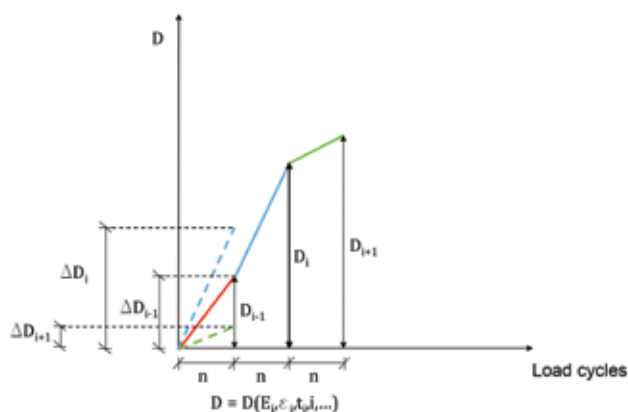
Figure 1: Incremental calculation and accumulation of damage according to Miner's rule. The incremental damage at the calculation step i - 1 is equal to \Delta D_{i-1} = \frac{n}{N_{Fi-1}} . In the calculation step i the incremental damage becomes \Delta D_i = \frac{n}{N_{Fi}} where, N_{Fi-1} \neq N_{Fi} , and the total damage is equal to D = \sum_{i=1}^j \Delta D_i ( t = temperature, i = increment, e = critical strain)
