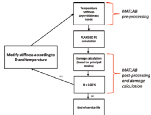
Figure 3: Implemented procedure for estimating service life (fatigue) with MATLAB (main routine) and PLAXIS 3D (subroutine)
