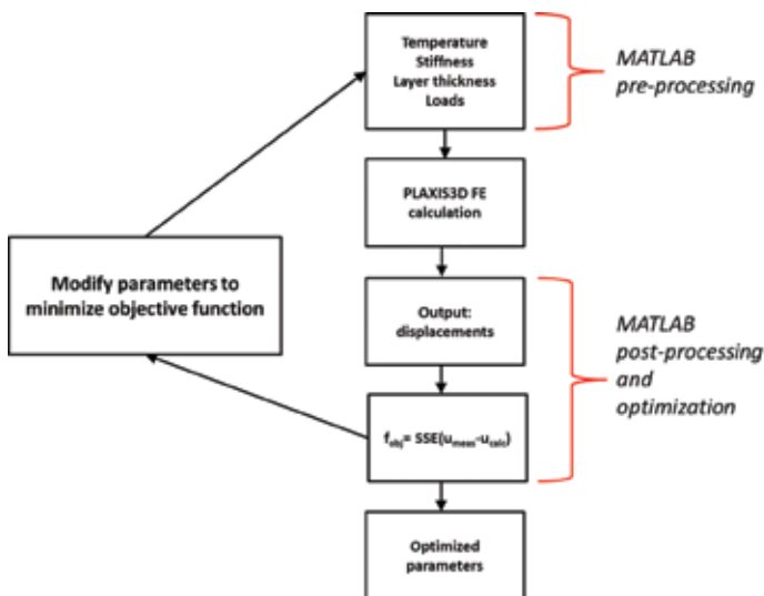
Figure 6: Inverse analysis procedure, coupling MATLAB (main routine) and PLAXIS 3D (subroutine)
