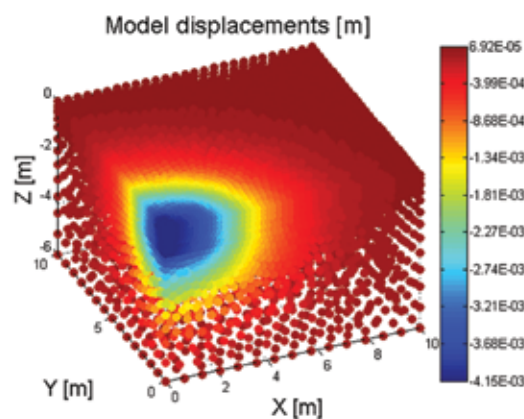
Figure 4b: MATLAB post-processing of pavement displacements calculated with PLAXIS 3D
