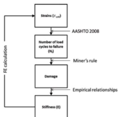
Figure 2: Simulation of the damage process due to fatigue in asphalt
